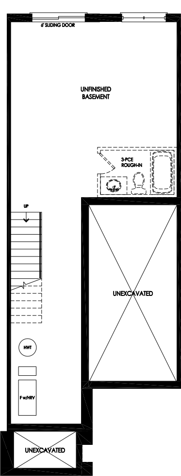
BASEMENT
