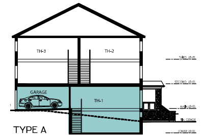
TYPE A CROSS SECTION
