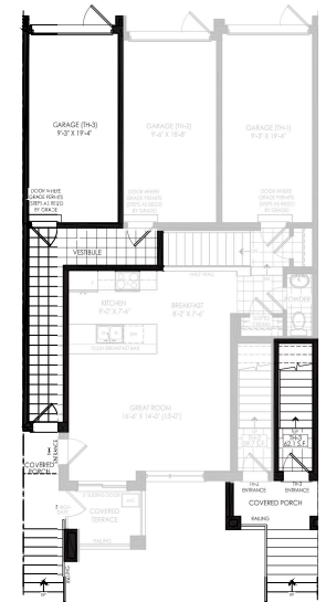
MAIN FLOOR TH-3
