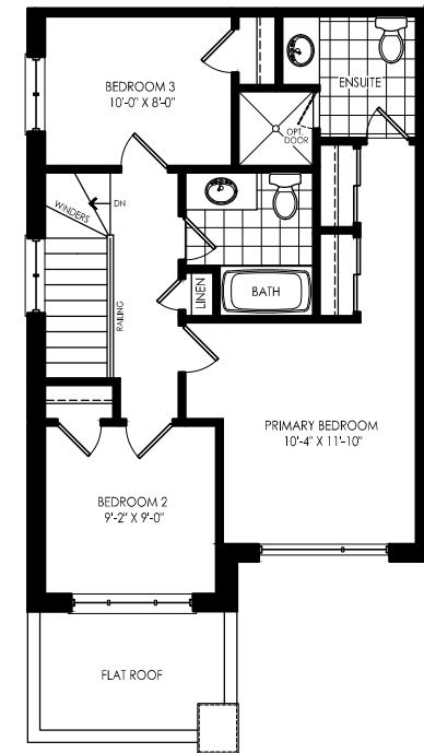
THIRD FLOOR
